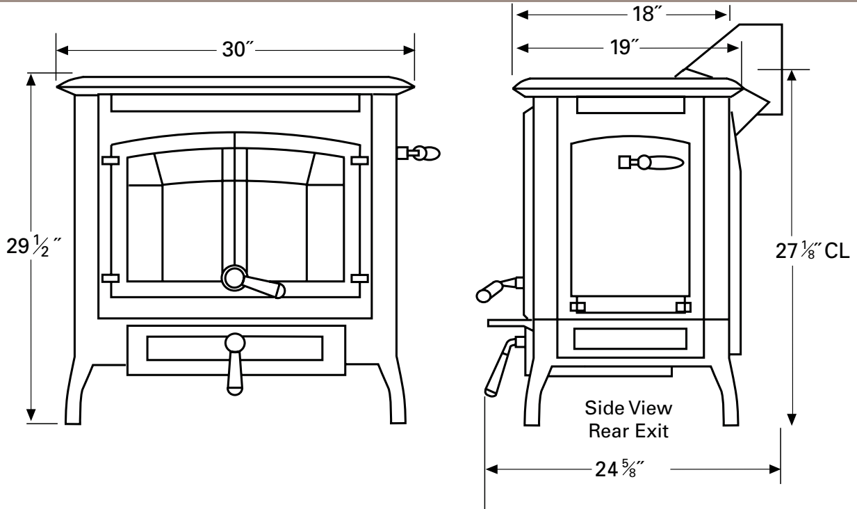
Minimum Hearthpad Dimensions Does not include the distance from the stove to the wall.
